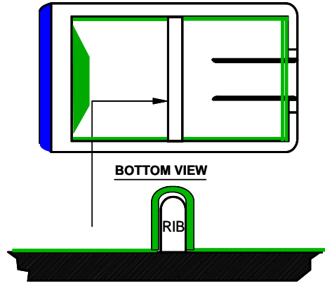
COVER BRACING RIB WITH FELT
